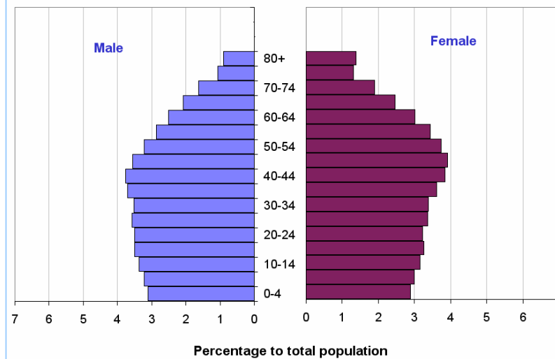
Figure 5 - Projected population pyramid : Kerala - 2026
