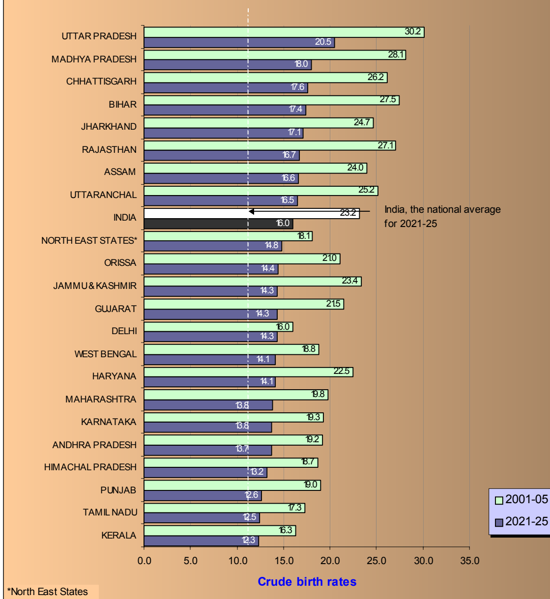
Figure-8 : Projected crude birth rates during 2001 - 2025, India and selected States
