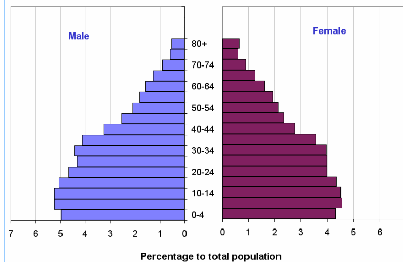
Figure 6 - Projected population pyramid : Uttar Pradesh - 2026
