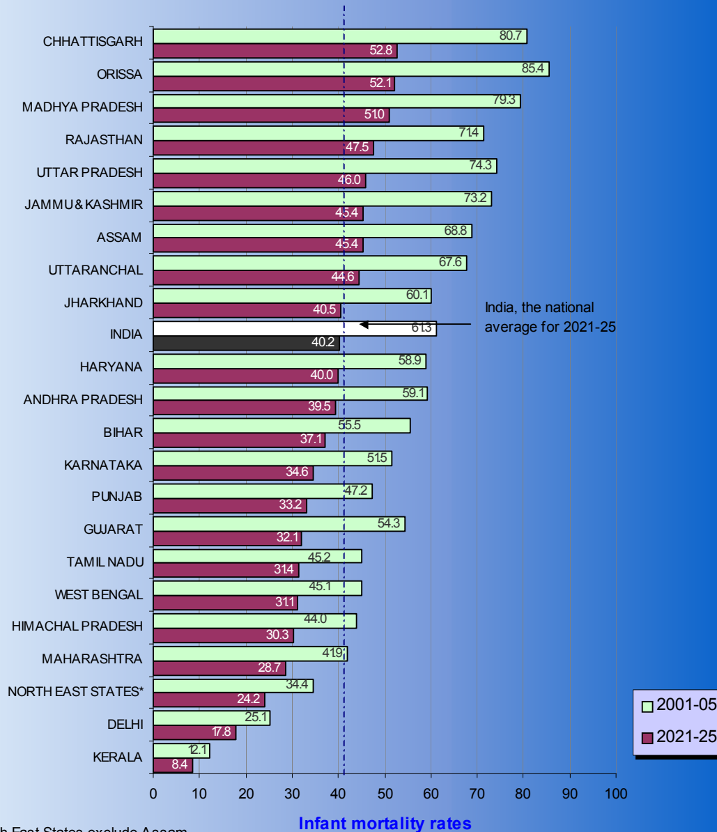
Figure-10 : Projected infant mortality rates during 2001- 2025, India and selected States
