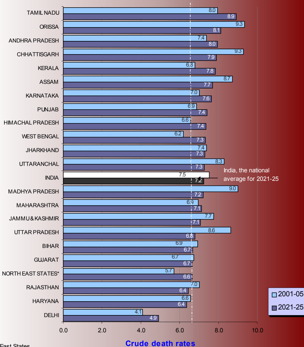
Figure-9 : Projected crude death rates during 2001 - 2025, India and selected States
